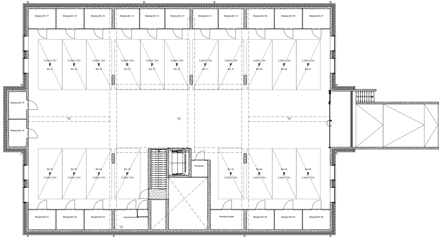
Kelder (garage)
